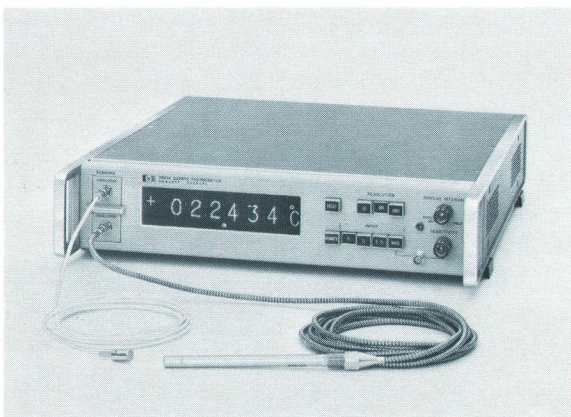
Fig. 4. A complete quartz thermometer system, the -hp- Model 2801A with two temperature sensing probes. With this system, the temperature of either probe or the difference between the temperatures of the two probes can be shown on the readout.
