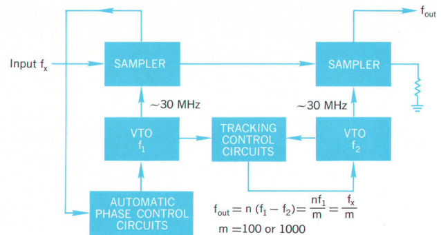
Fig. 2. Simplified block diagram of automatic frequency divider. Control circuits maintain indicated relationships between f_x , f_1 , and f_2 .
