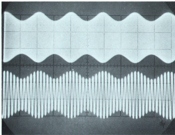
Fig. 7. For AM signals, frequency divider output tends to be a lower-frequency replica of the input. Traces show divider output for 1 GHz input signal, 20% amplitude modulated by 100 kHz signal. Top: divider output for division ratio m = 100 . Bottom: divider output for m = 1000 .
