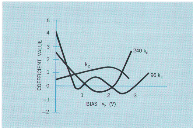
Fig. 5. Second, fourth, and sixth-power coefficients of hypothetical diode characteristic of Fig. 4. Biasing one diode of balanced mixer at 1V and the other at 2V makes k_6 's cancel and k_4 's = 0, but changes desired coefficient k_2 by only a few dB.
