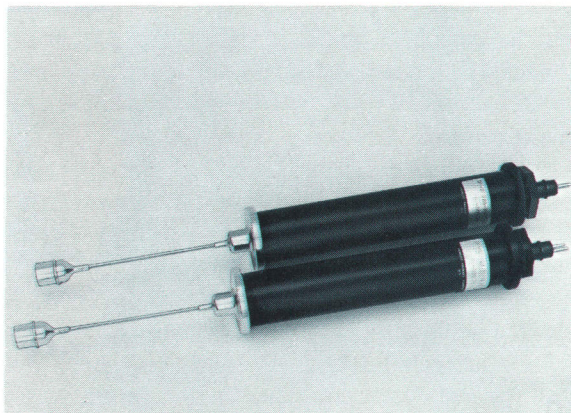
Fig. 5. Where a probe is used for precision measurements in still water, heat dissipated by the electronics in the package may heat the surrounding water, thus influencing the probe temperature. The modification shown here places the quartz crystal at some distance from the remainder of the probe and minimizes this effect.
