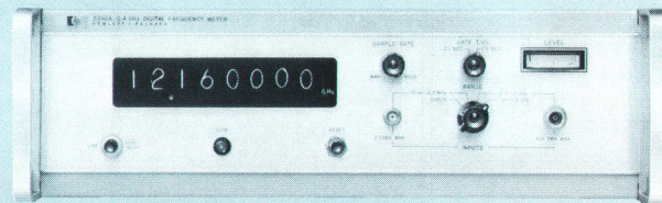
-hp- 5240A 12.4 GHz Digital Frequency Meter
